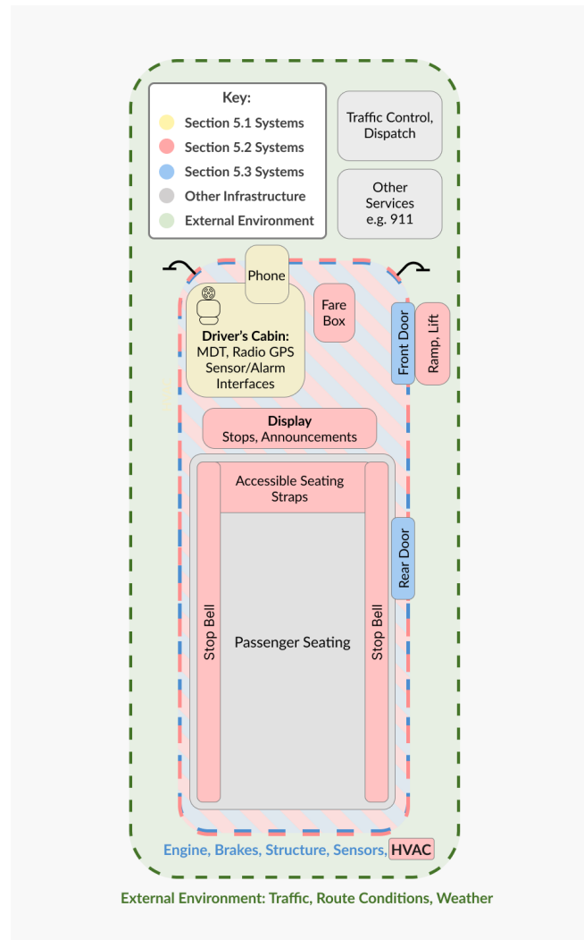
Figure 1: Generalized bus diagram illustrating the approximate spatial layout of systems described in the Findings. This generalized layout is not to scale and is not intended as an exact depiction of any particular vehicle model.
